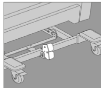
Rocker/Lock Mechanism
