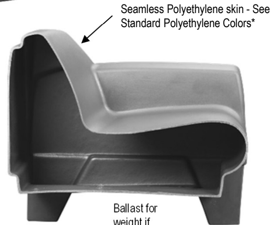
Cross-section of rotationally molded plastic lounge chair
