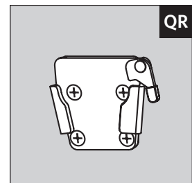
Additional Quick Release Accessory Bracket Additional attachment bracket for IV Pole and other various accessories. (Options requiring QR Bracket include the necessary bracket/hardware) Mounted into metal insert nuts in recliner arm.
